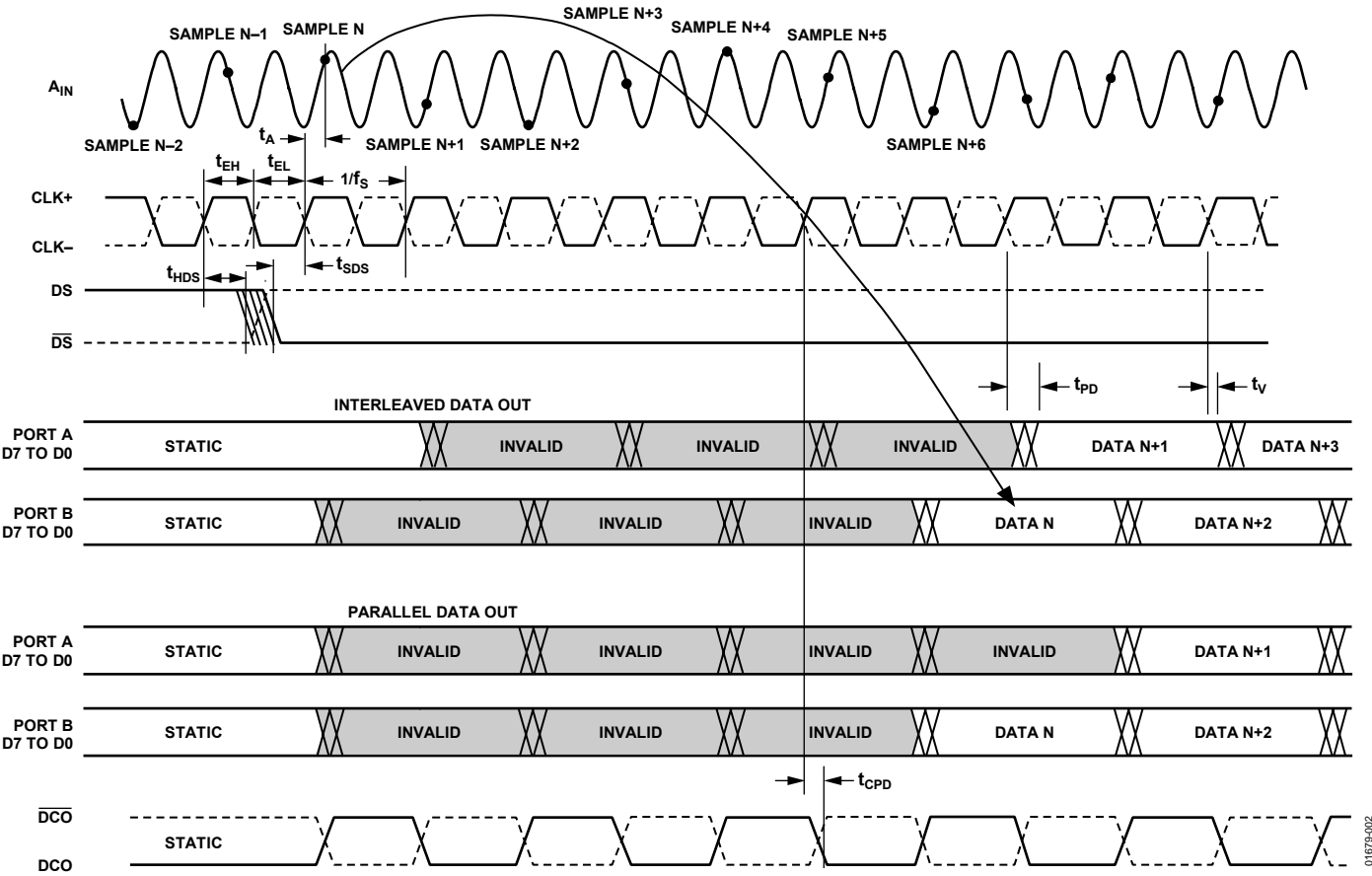
Figure 2. Timing Diagram
