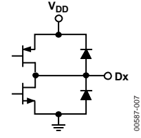
Figure 24. Digital Output Circuit
