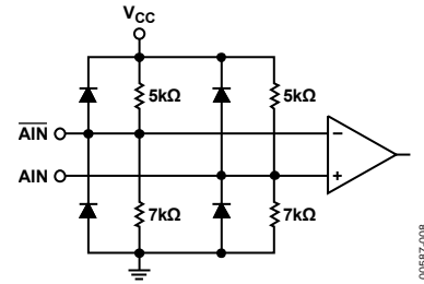
Figure 25. Analog Input Circuit
