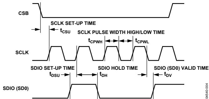
Figure 6. SPI Timing Diagram
