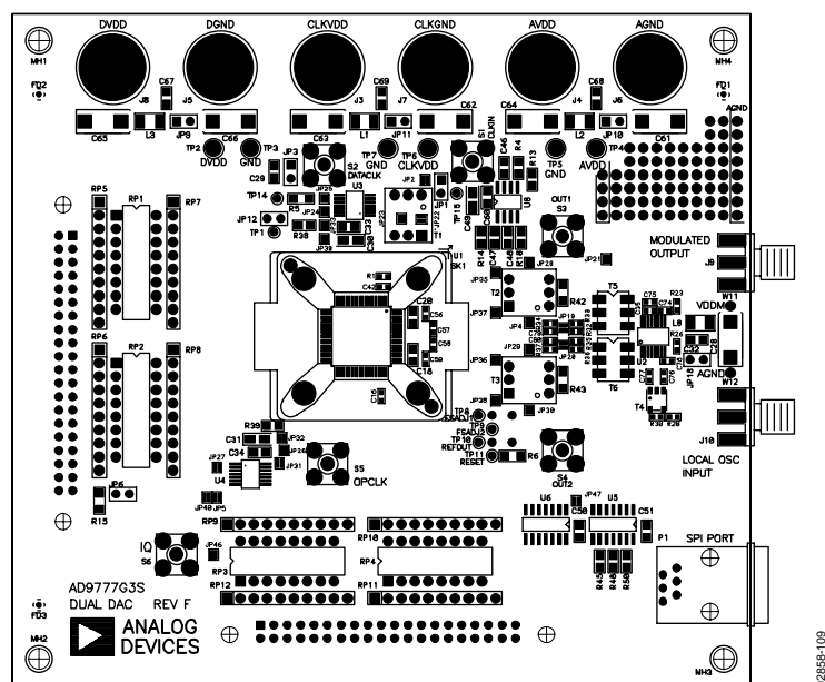
Figure 109. AD9775 Evaluation Board Components, Top Side
