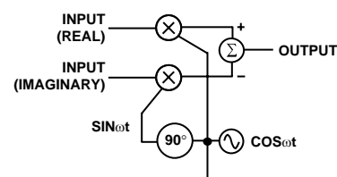
Figure 78. Quadrature Modulator
