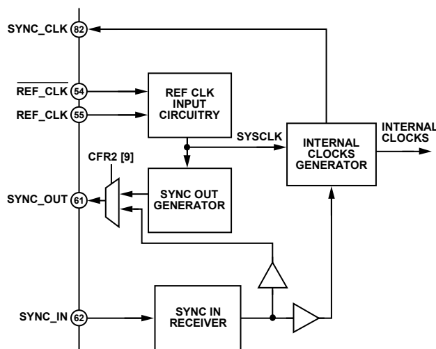
Figure 48. Synchronization Block Diagram
