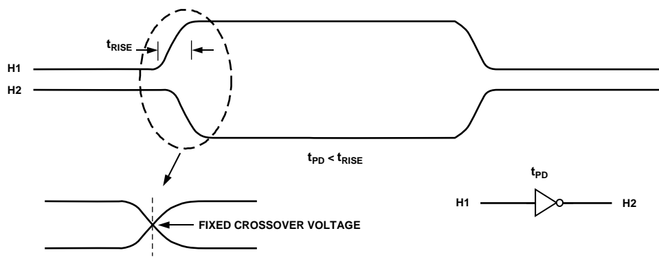
Figure 18. H-Clock Inverse Phase Relationship
