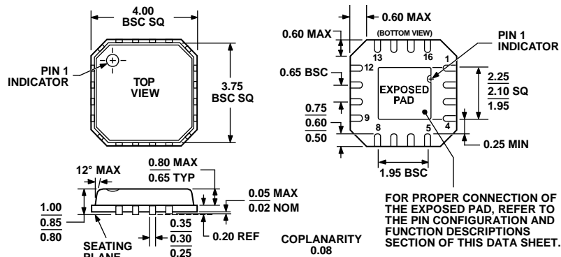
Figure 23. 16-Lead Lead Frame Chip Scale Package [LFCSP_VQ]
