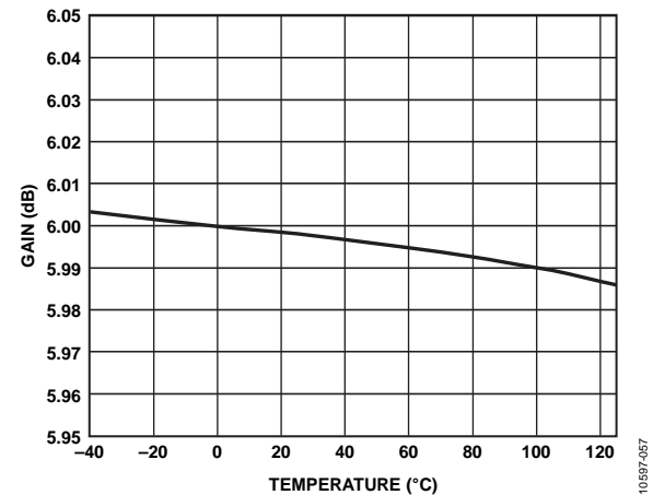
Figure 14. DC Pass Band Gain Drift (-40°C to +125°C)
