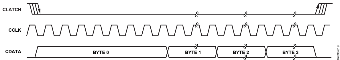
Figure 19. SPI Write Cloning (Single-Write Mode)
