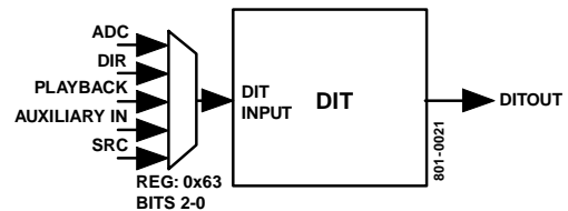
Figure 20. Digital Output Transmitter Block Diagram
