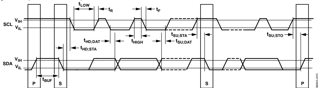
Figure 23. SMBus Interface
