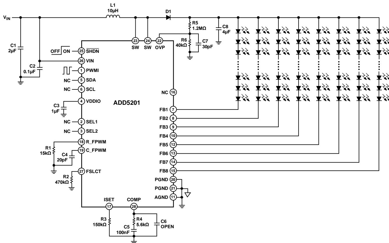
Figure 29. Typical Application Circuits for PWM Interface with Phase Shift PWM Dimming Mode
