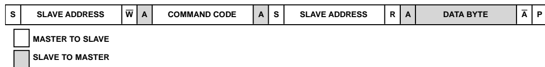
Figure 24. Read Byte Protocol
