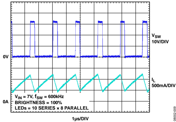
Figure 10. Switching Waveforms, V_{IN} = 7\text{ V}
