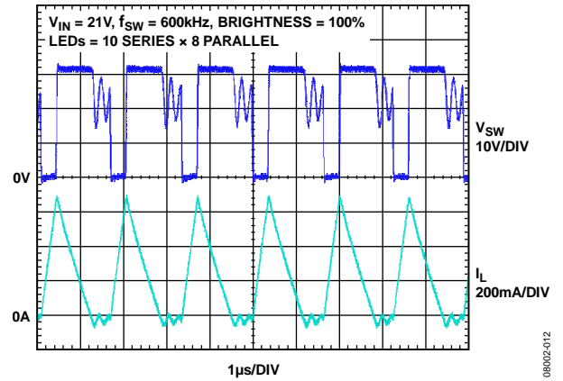
Figure 13. Switching Waveforms, V_{IN} = 21\text{ V}
