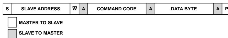
Figure 25. Write Byte Protocol
