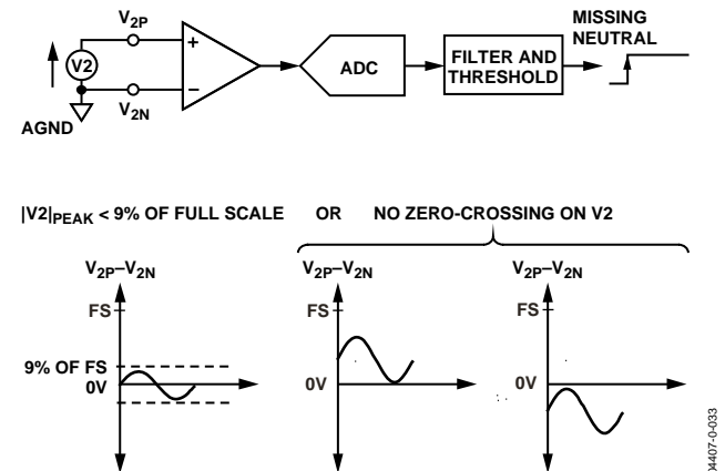
Figure 31. Missing Neutral Detection
