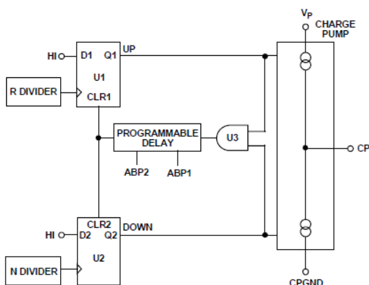
Figure 7. PFD Simplified Schematic and Timing (in Lock)
