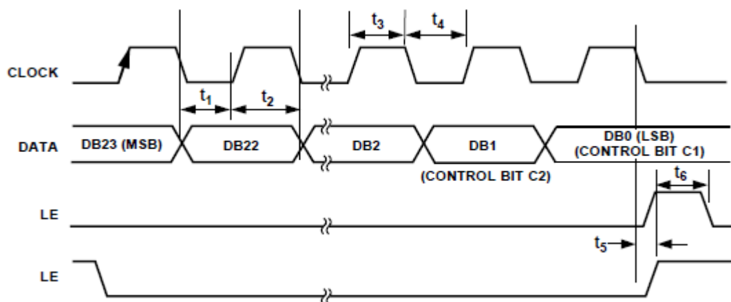
Figure 2 – Timing Diagram.
