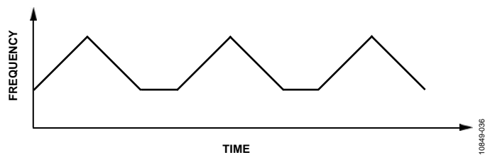
Figure 43. Delay Between Ramps for Triangular Mode
