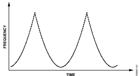
Figure 46. Parabolic Ramp
