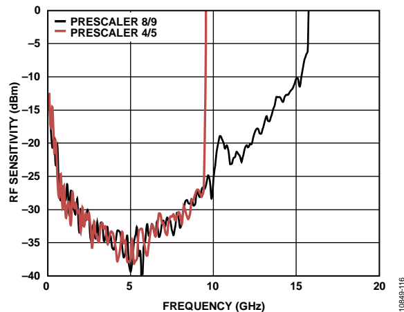
Figure 16. RF IN Sensitivity at Nominal Temperature
