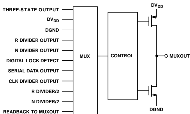
Figure 22. MUXOUT Schematic
