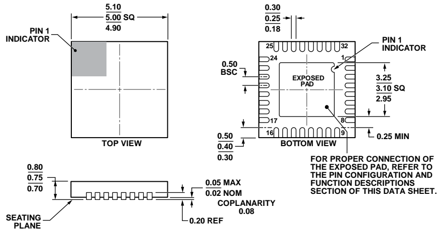
Figure 39. 32-Lead Lead Frame Chip Scale Package [LFCSP_WQ] 5 mm × 5 mm Body, Very Very Thin Quad (CP-32-7)
