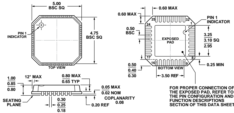
Figure 40. 32-Lead Lead Frame Chip Scale Package [LFCSP_VQ] 5 mm × 5 mm Body, Very Thin Quad (CP-32-2)
