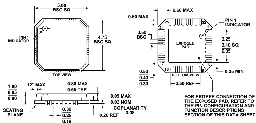
COMPLIANT TO JEDEC STANDARDS MO-220-VHHD-2 Figure 40. 32-Lead Lead Frame Chip Scale Package [LFCSP_VQ] 5 mm x 5 mm Body, Very Thin Quad (CP-32-2) Dimensions shown in millimeters
