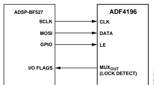
Figure 39. ADSP-BF527-to-ADF4196 Interface
