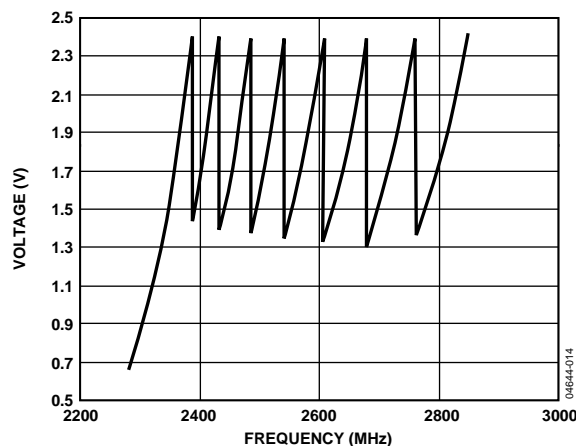
Figure 14. Frequency vs. V_{TUNE} ADF4360-0
