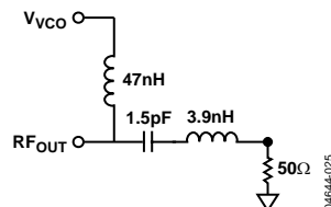
Figure 21. Differential ADF4360-0 Output Stage
