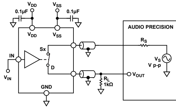
Figure 29. THD + Noise
