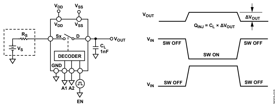
Figure 33. Charge Injection
