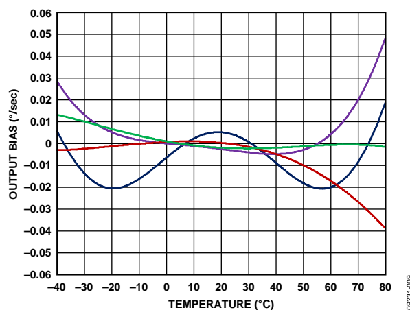
Figure 9. Bias vs. Temperature, 0.1°C/Minimum Ramp Rate, Autotune at 25°C, SMPL_PRD = 0x001F, and DEC_RATE = 0x0010
