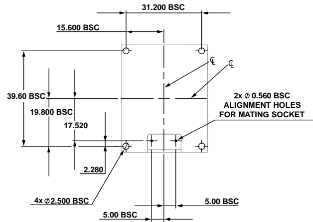
Figure 23. Suggested Mounting Hole Locations, Connector Down
