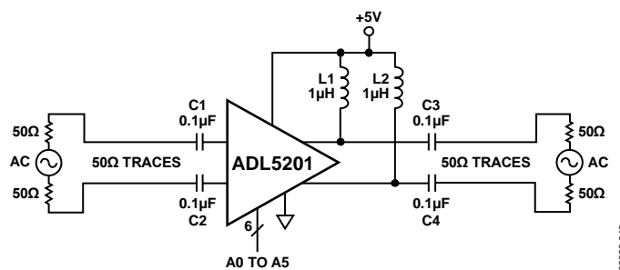
Figure 46. Test Circuit for S-Parameters on Dedicated 50 Ω Differential-to-Differential Board
