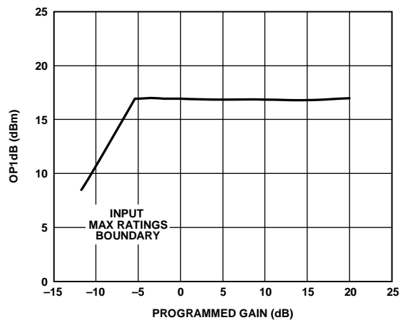
Figure 20. OP1\text{dB} vs. Programmed Gain at 140 MHz, Low Power Mode
