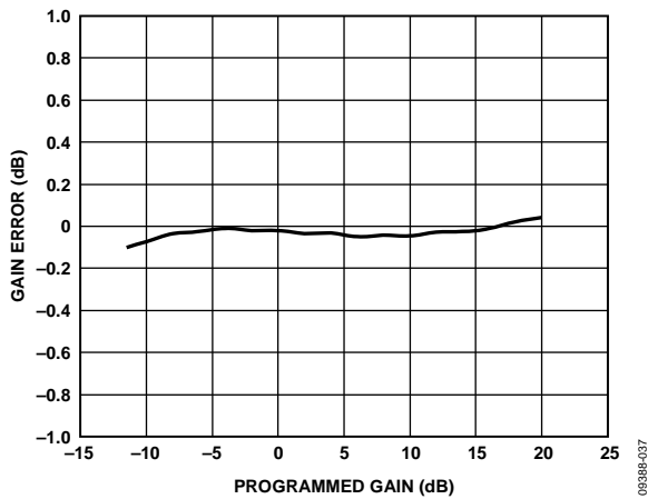
Figure 38. Gain Step Error, Frequency = 140 MHz
