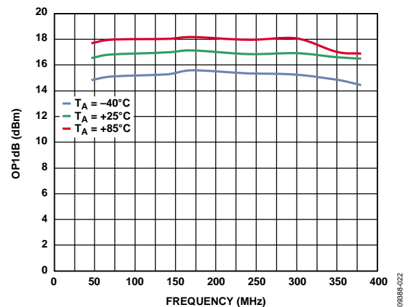
Figure 23. OP1\text{dB} vs. Frequency at Maximum Gain, Three Temperatures, Low Power Mode
