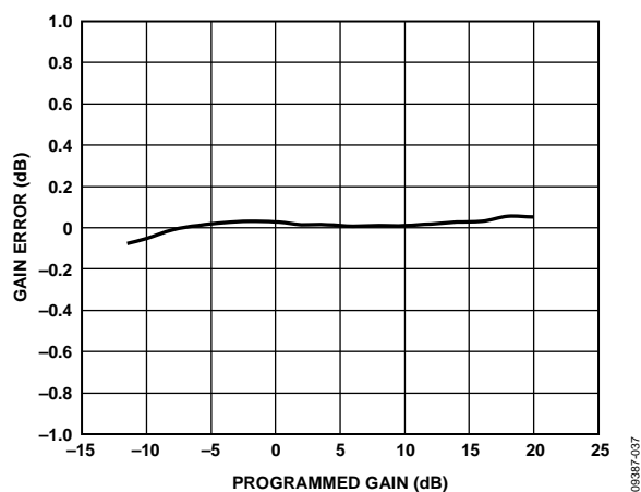
Figure 38. Gain Step Error, Frequency = 140 MHz
