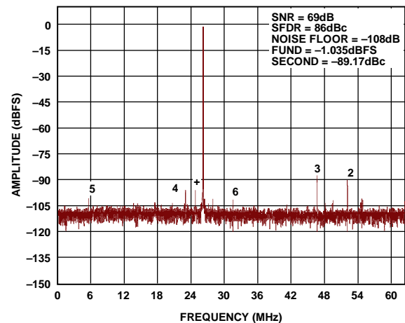
Figure 57. Measured Single-Tone Performance of the Circuit in Figure 55 for a 100 MHz Input Signal
