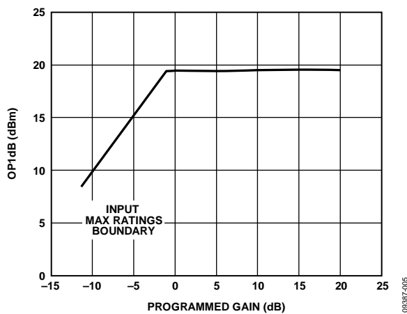
Figure 8. OP1dB vs. Programmed Gain at 140 MHz
