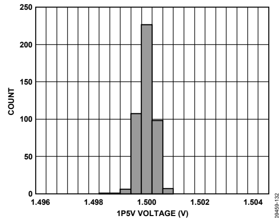
Figure 32. 1P5V Histogram
