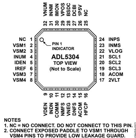
Figure 2. 32-Lead LFCSP Pin Configuration
