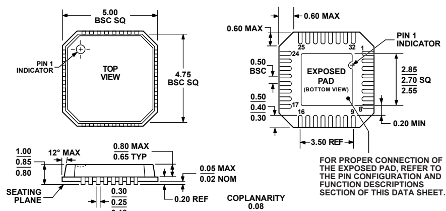
Figure 61. 32-Lead Lead Frame Chip Scale Package [LFCSP_VQ] 5 mm x 5 mm Body, Very Thin Quad (CP-32-8) Dimensions shown in millimeters
