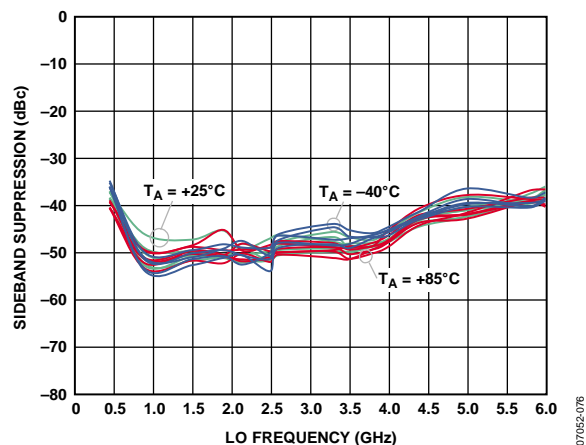
Figure 36. Sideband Suppression vs. LO Frequency ( f_{LO} ) and Temperature; Multiple Devices Shown
