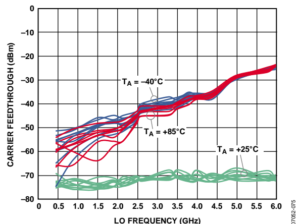
Figure 35. Carrier Feedthrough vs. LO Frequency ( f_{LO} ) and Temperature After Nulling at 25°C; Multiple Devices Shown
