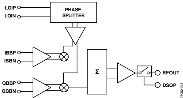
Figure 53. Block Diagram
