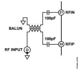
Figure 81. RF Input
