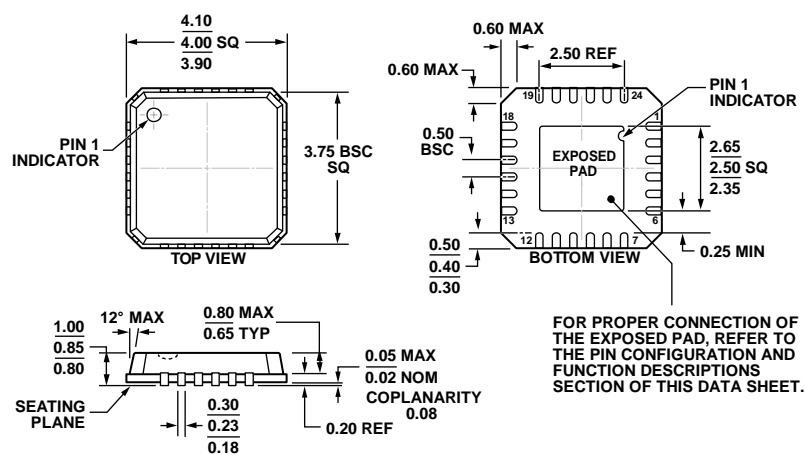
Figure 105. 24-Lead Lead Frame Chip Scale Package [LFCSP_VQ] 4 mm × 4 mm Body, Very Thin Quad (CP-24-3) Dimensions shown in millimeters
