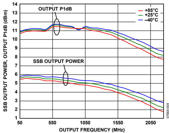
Figure 4. Single Sideband (SSB) Output Power ( P_{\text{OUT}} ), Output P1 dB vs. Output Frequency and Temperature
