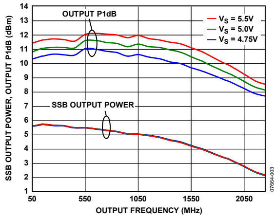
Figure 3. Single Sideband (SSB) Output Power ( P_{\text{OUT}} ), Output P1dB vs. Output Frequency and Power Supply
