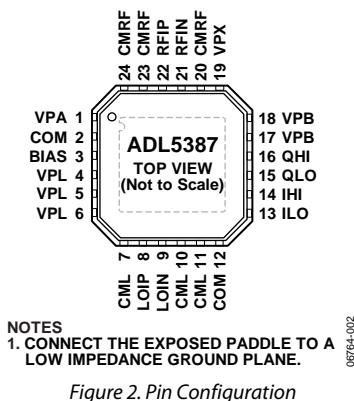
Figure 2. Pin Configuration
