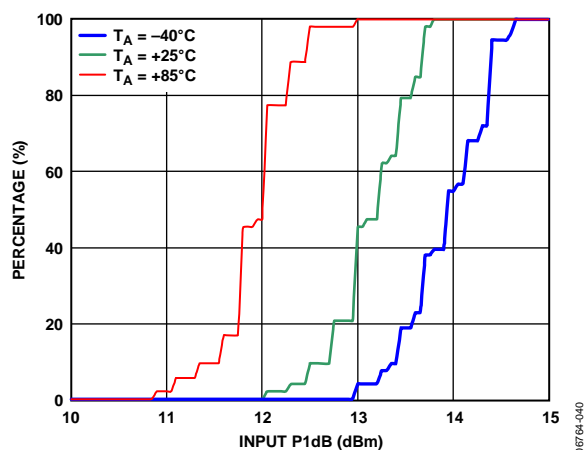
Figure 40. IP1dB Distributions
