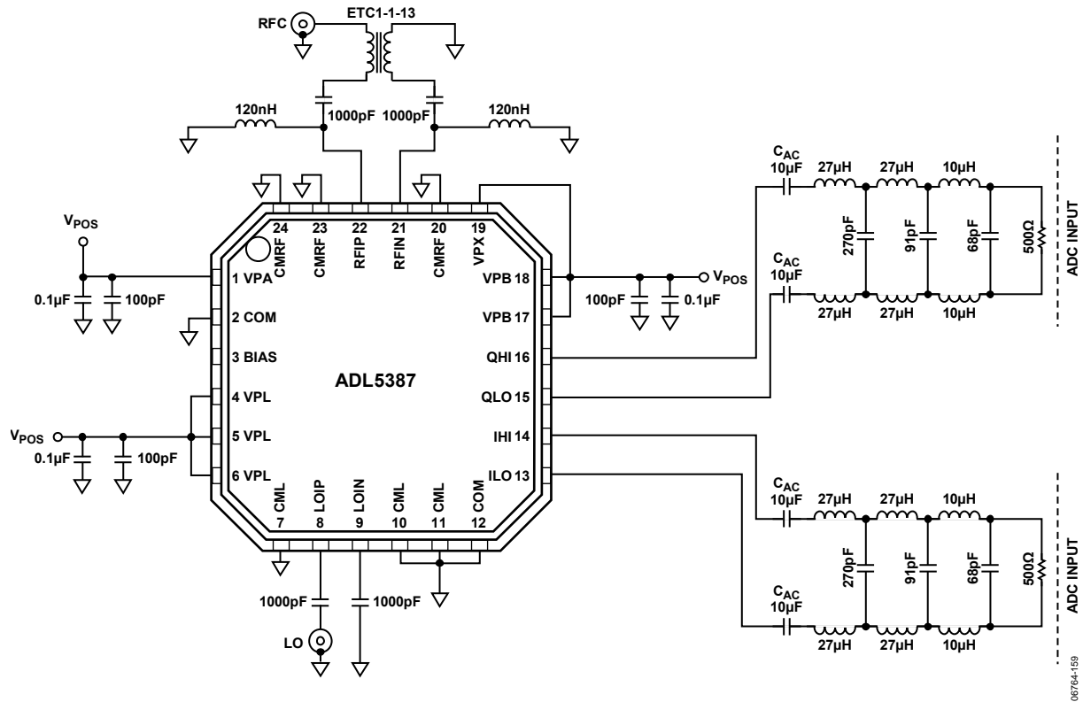
Figure 59. Sixth Order Low-Pass Butterworth Baseband Filter Schematic
