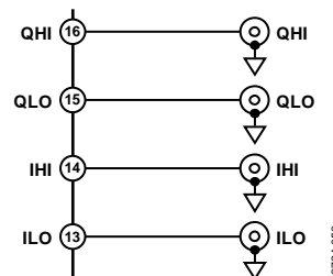
Figure 50. Baseband Output Configuration
