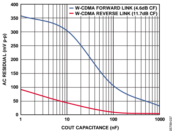
Figure 37. AC Residual vs. C OUT , W-CDMA Reverse Link (11.7 dB CF) Waveform and W-CDMA Forward Link (4.6 dB CF) Waveform
