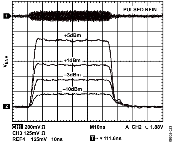
Figure 40. V_{ENV} Output Response to Various RF Input Pulse Levels 900 MHz Frequency
