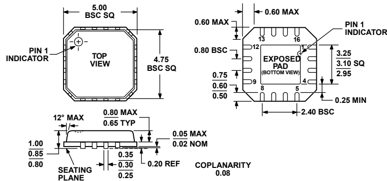
Figure 26. 16-Lead Lead Frame Chip Scale Package [LFCSP_VQ] 5 mm x 5 mm Body, Very Thin Quad CP-16-6 Dimensions shown in millimeters
