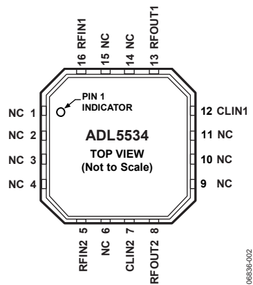
Figure 2. Pin Configuration
