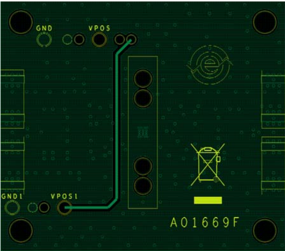
Figure 25. Evaluation Board Layout (Bottom)
