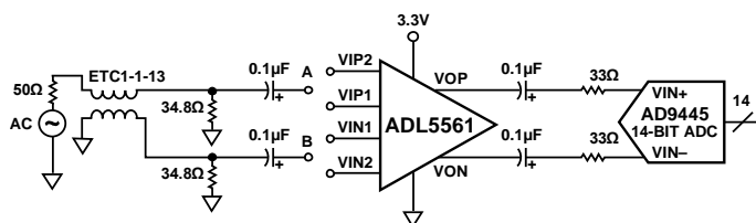
Figure 39. Wideband ADC Interfacing Example Featuring the AD9445
