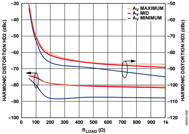
Figure 21. Harmonic Distortion (HD2/HD3) vs. R_{LOAD}
