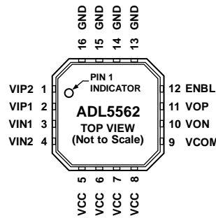
Figure 2. Pin Configuration
