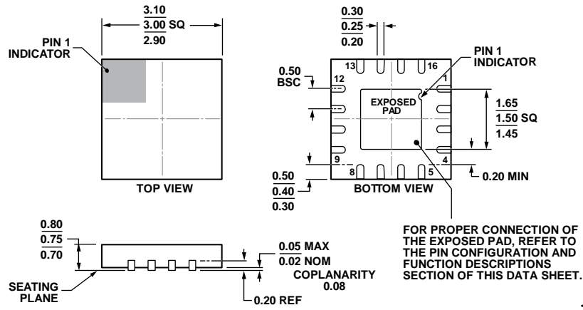
Figure 48. 16-Lead Lead Frame Chip Scale Package [LFCSP_WQ] 3 mm × 3 mm Body, Very Very Thin Quad (CP-16-27)
