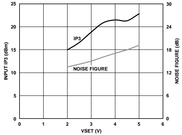
Figure 57. Input IP3, Noise Figure vs. VSET
