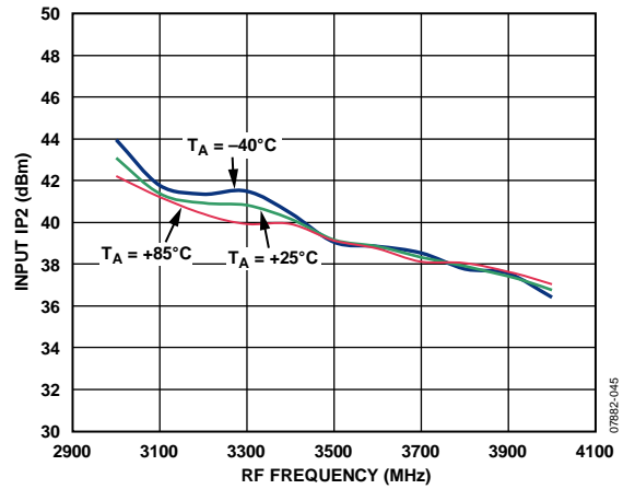
Figure 45. Input IP2 vs. RF Frequency
