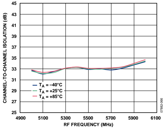
Figure 66. Channel-to-Channel Isolation
