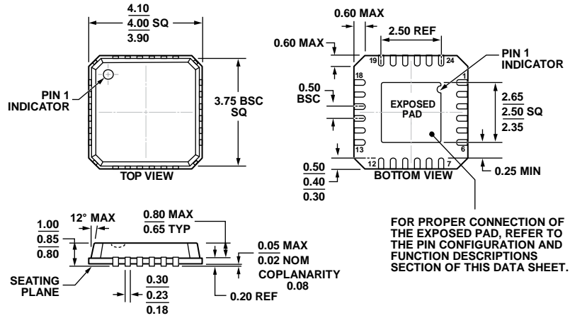
Figure 76. 24-Lead Lead Frame Chip Scale Package [LFCSP_VQ] 4 mm × 4 mm Body, Very Thin Quad (CP-24-3) Dimensions shown in millimeters
