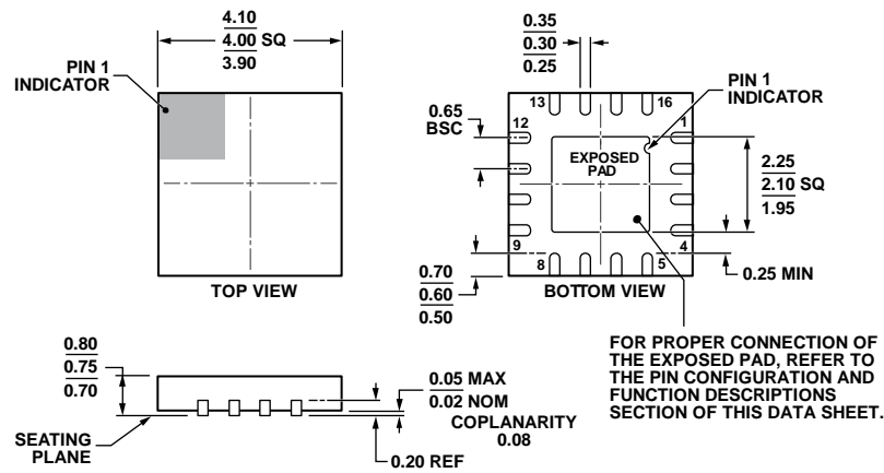
Figure 66. 16-Lead Lead Frame Chip Scale Package [LFCSP_WQ] 4 mm × 4 mm Body, Very Very Thin Quad (CP-16-23) Dimensions shown in millimeters
