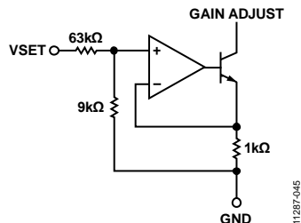
Figure 47. VSET Interface Simplified Schematic
