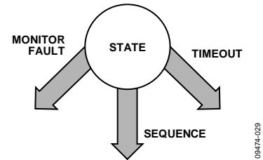
Figure 19. State Cell
