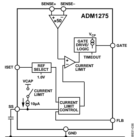
Figure 54. Soft Start
