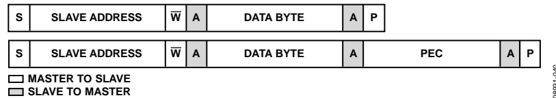
Figure 58. Send Byte and Send Byte with PEC
