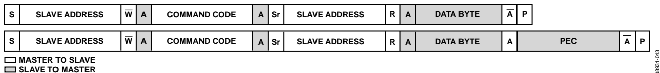
Figure 61. Read Byte and Read Byte with PEC
