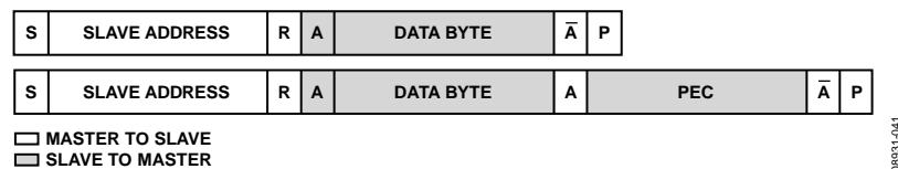
Figure 59. Receive Byte and Receive Byte with PEC
