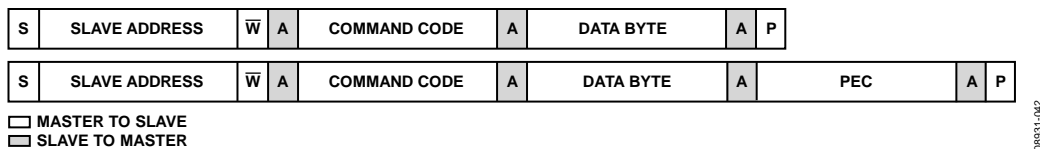
Figure 60. Write Byte and Write Byte with PEC
