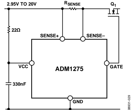
Figure 47. Transient Glitch Protection Using an RC Network
