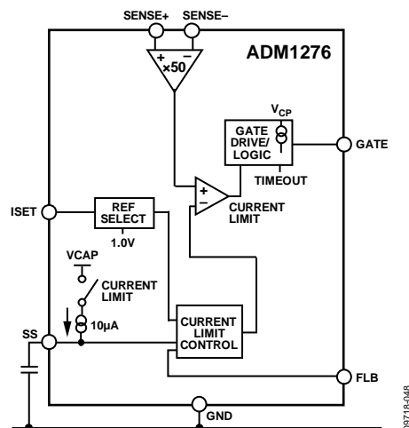
Figure 48. Soft Start
