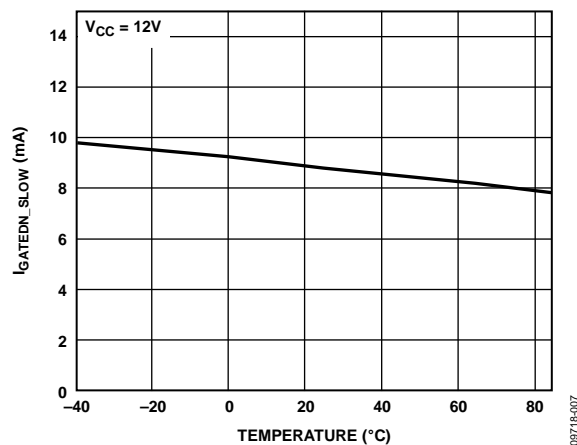
Figure 7. Gate Pull-Down Current ( I_{GATEDN\_SLOW} ) vs. Temperature
