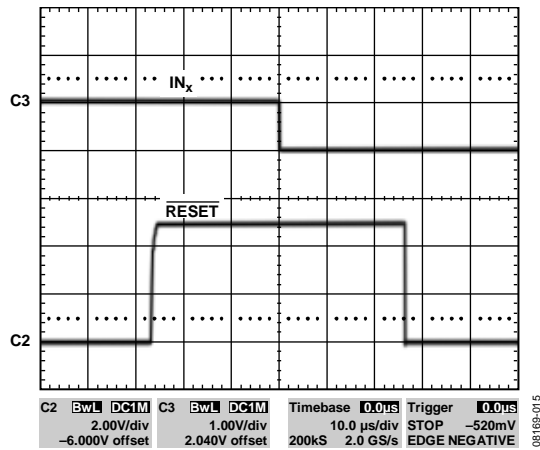
Figure 9. RESET Pull-Up and Pull-Down Response (10 µs/Div)
