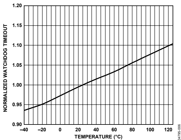
Figure 6. Normalized Watchdog Timeout Period vs. Temperature
