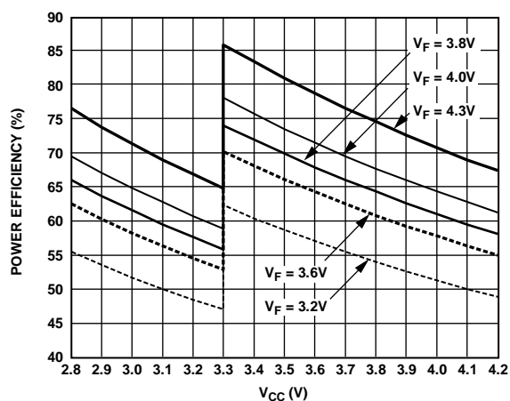
Figure 17. Power Efficiency vs. Supply Voltage over Li-Ion Range, Four LEDs @ 15 mA/LED
