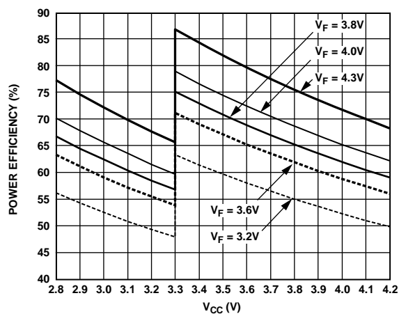
Figure 16. Power Efficiency vs. Supply Voltage over Li-Ion Range, Six LEDs @ 15 mA/LED
