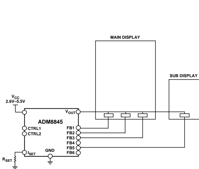
Figure 29. Driving Three Main LEDs and One Sub LED
