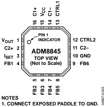
Figure 2. Pin Configuration
