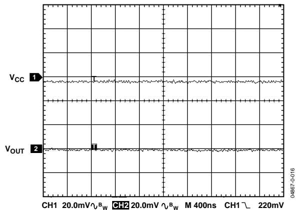
Figure 15. 1x Mode Operating Waveforms
