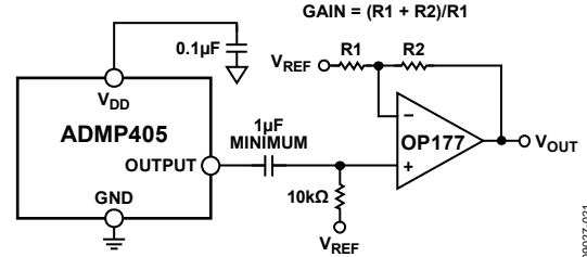
Figure 8. ADMP405 Connected to the OP177 Op Amp
