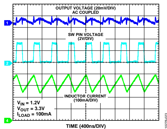
Figure 23. Typical PWM Mode Operation, I_{LOAD} = 100mA
