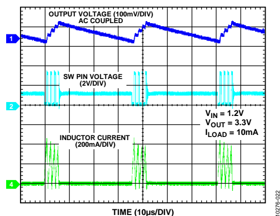
Figure 22. Typical PFM Mode Operation, I_{LOAD} = 10mA
