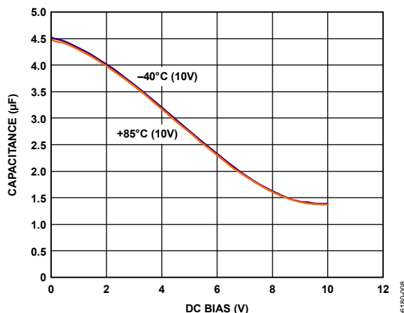
Figure 33. DC Bias Characteristic of a 10V, 4.7 \mu F Ceramic Capacitor
