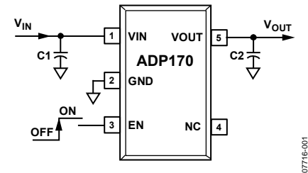
Figure 1. ADP170 with Fixed Output Voltage, 1.8 V
