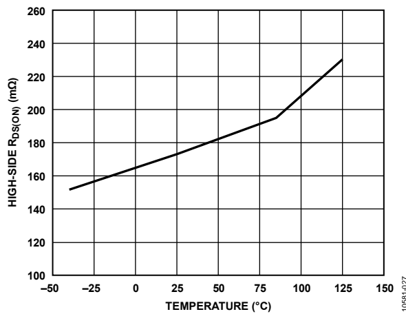
Figure 24. High-Side R_{DS(ON)} vs. Temperature
