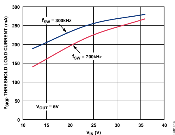
Figure 14. Pulse Skip Threshold, V_{OUT} = 5V
