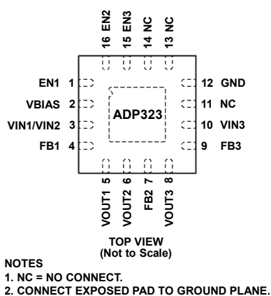
Figure 4. ADP323 Pin Configuration
