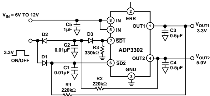
Figure 22. Turn-On/Turn-Off Sequencing for Mixed Supply Voltages
