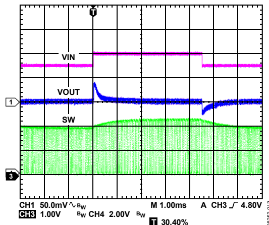
Figure 27. Buck2 Response to Line Transient, V_{IN} = 4.5\text{ V} to 5.0\text{ V} , V_{OUT2} = 1.8\text{ V} , PWM Mode
