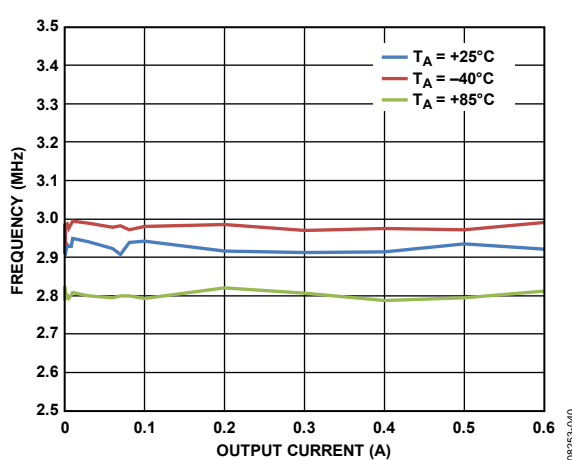
Figure 21. Buck2 Switching Frequency vs. Output Current, Across Temperature, VOUT2 = 1.8 V, PWM Mode
