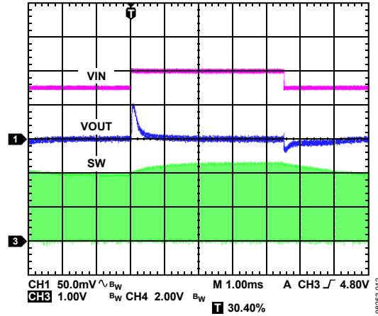
Figure 26. Buck1 Response to Line Transient, Input Voltage from 4.5\text{ V} to 5.0\text{ V} , V_{OUT1} = 3.3\text{ V} , PWM Mode
