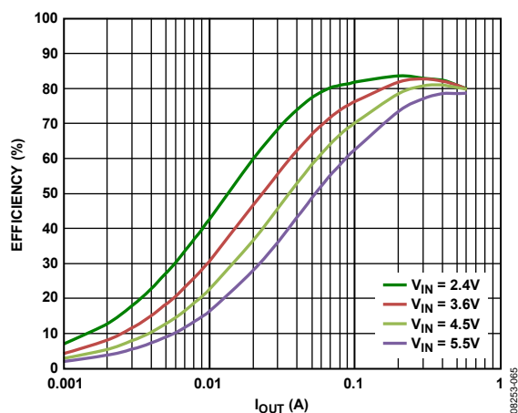
Figure 18. Buck1 Efficiency vs. Load Current, Across Input Voltage, VOUT1 = 0.8 V, PWM Mode
