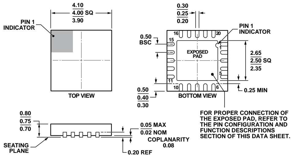
Figure 70. 20-Lead, Lead Frame Chip Scale Package [LFCSP_WQ] 4 mm × 4 mm Body, Very Very Thin Quad (CP-20-10)
