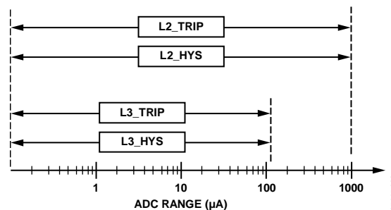
Figure 32. Comparator Ranges
